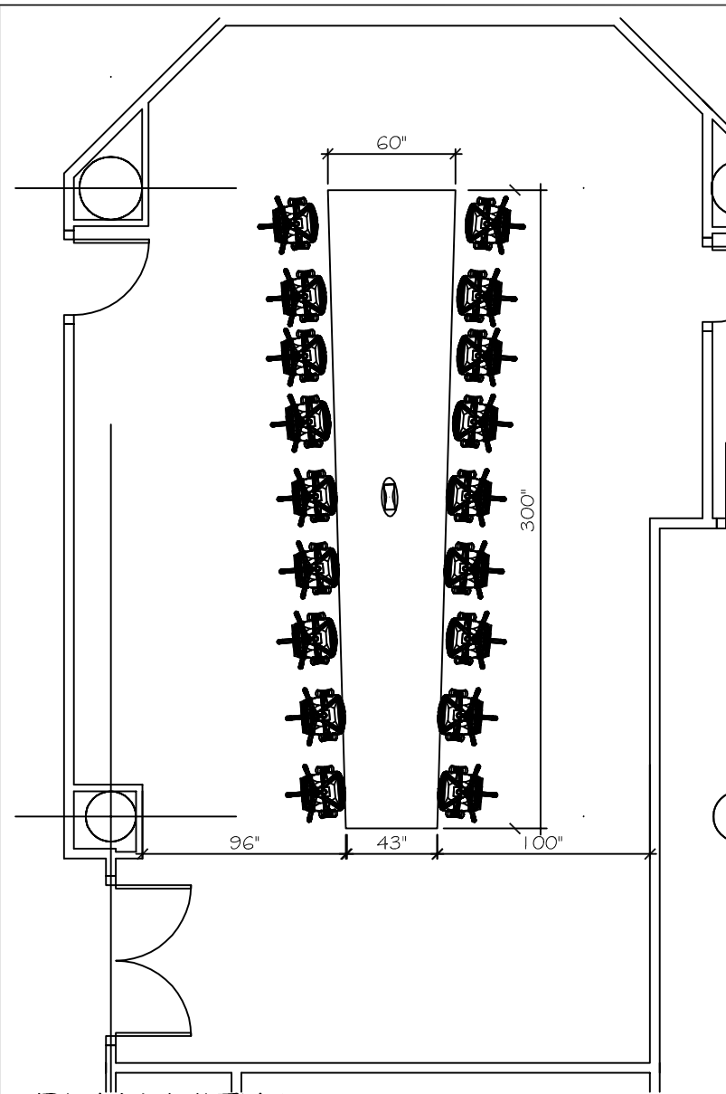
PLAN VIEW
